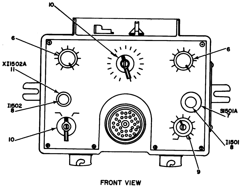
Figure 21. Radio Set Control C-1439/U (Sheet 1 of 2).
