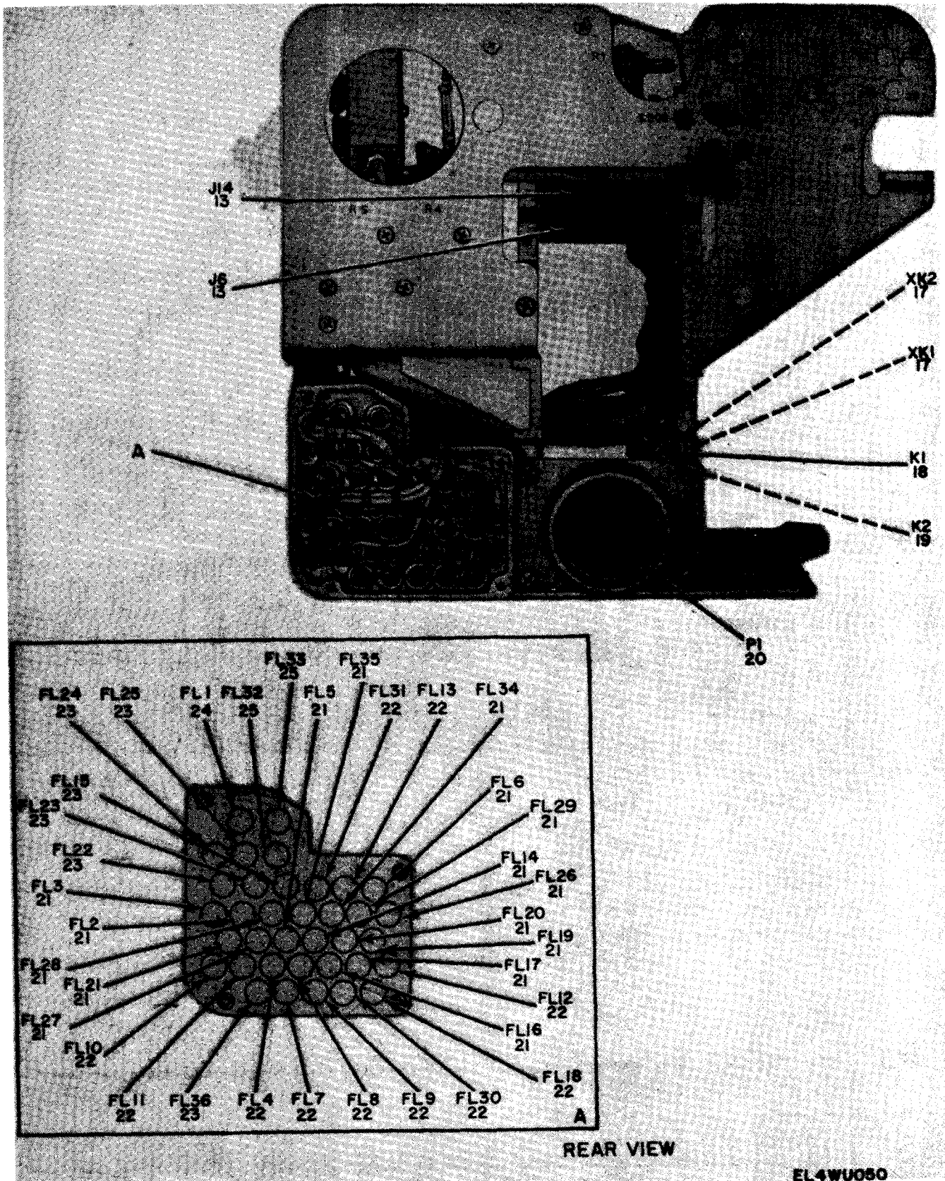
Figure 31. Receiver-Transmitters RT-441/TRC-68 and RT-441A/TRC-68, Main Frame (Sheet 2 of 2).
