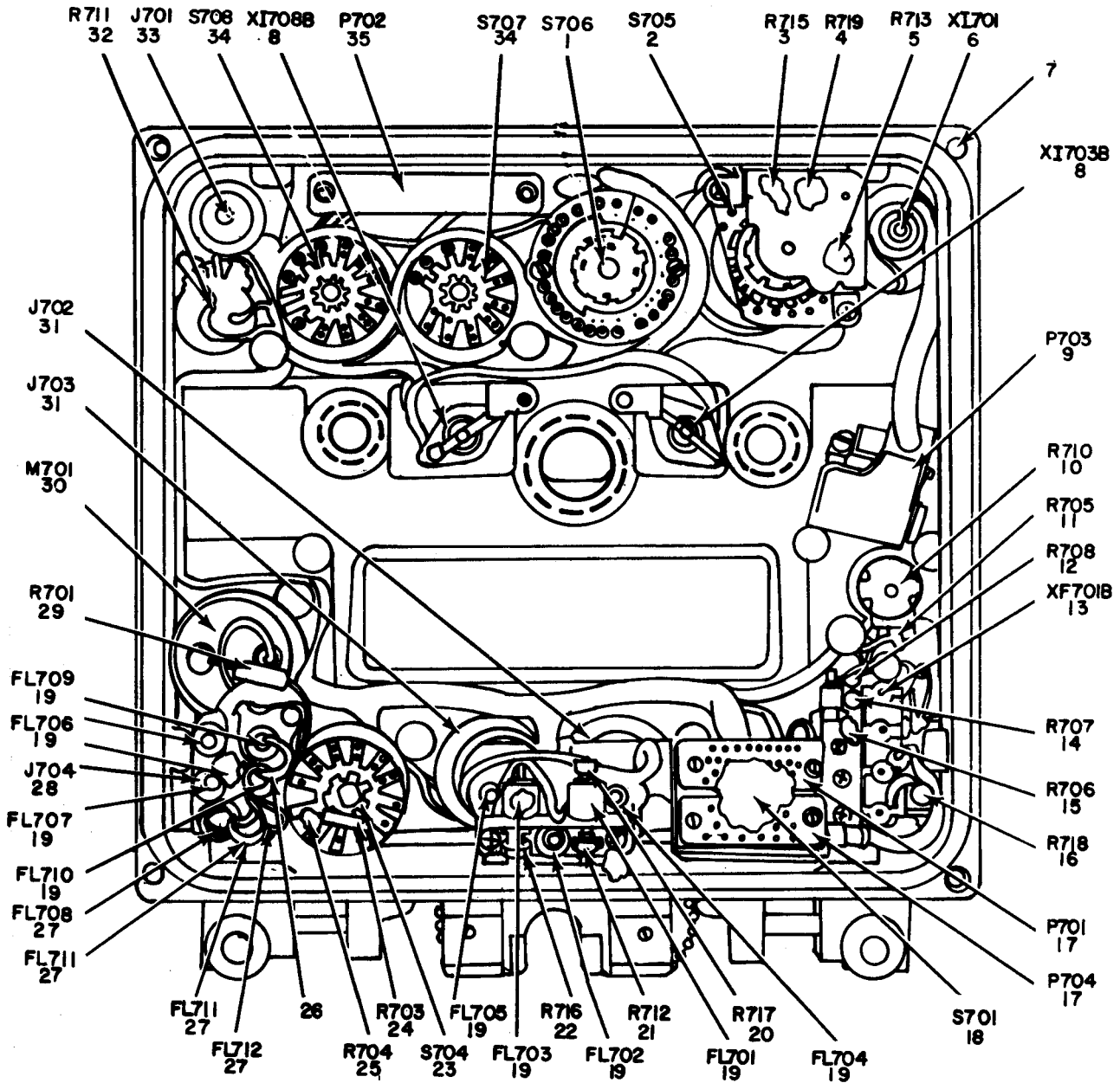
Figure 30. Receiver-Transmitters RT-441/TRC-68 and RT-441A/TRC-68 Front Panel, Rear View.
