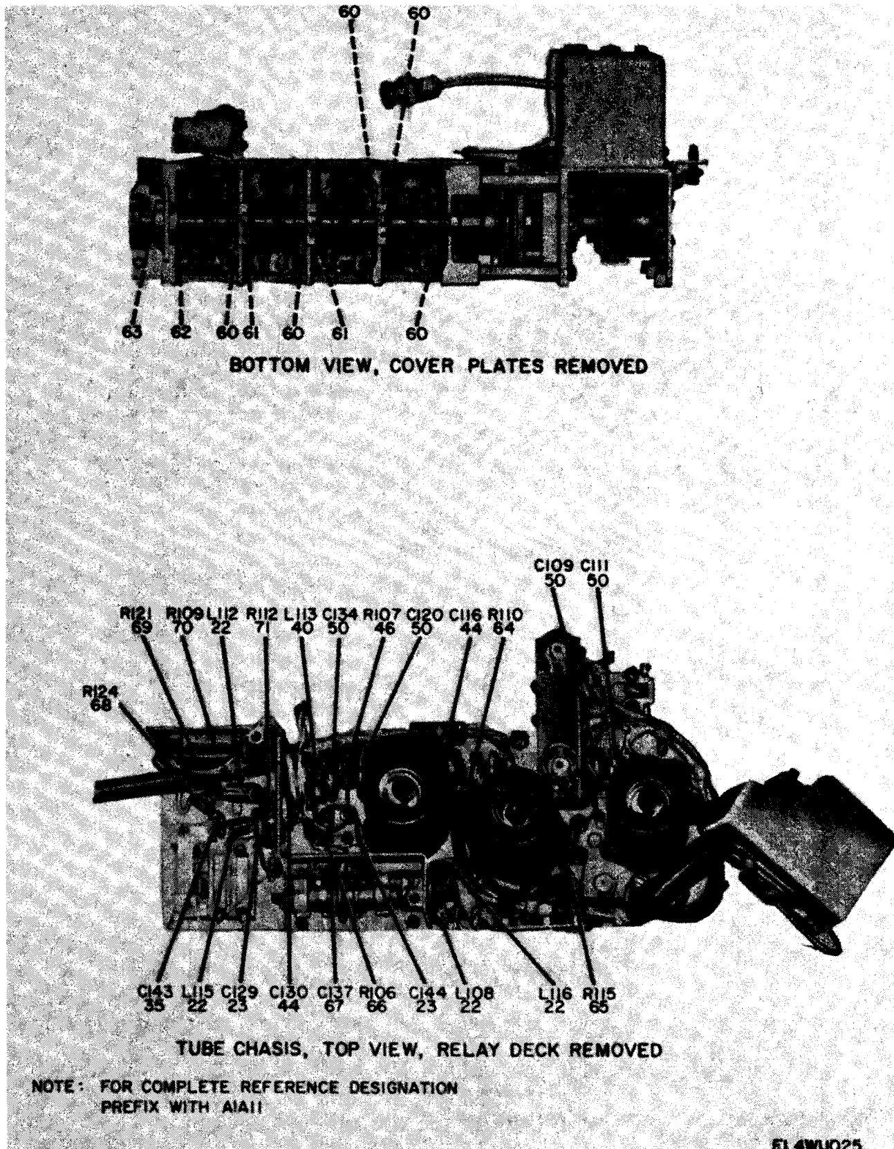
Figure 14. RF Power Amplifier 225 to 399.9 MHz Subunit (A1A11) (Sheet 3 of 3).
