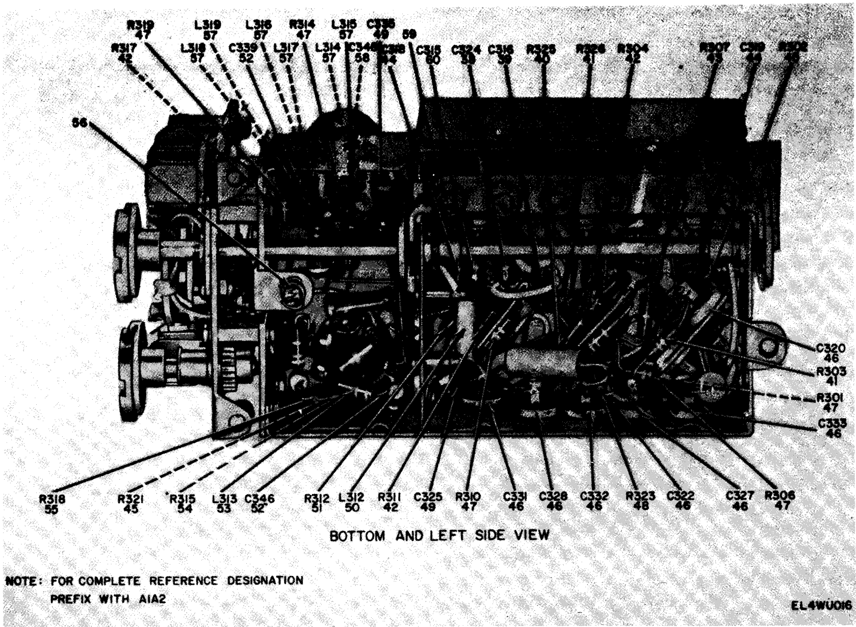
Figure 11. First IF Amplifier 20 to 29.9 MHz Subunit (A1A2) (Sheet 2 of 3).
