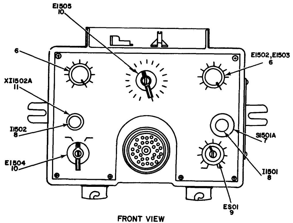
Figure 43. Radio Set Control C-1439/U (Sheet 1 of 2).
