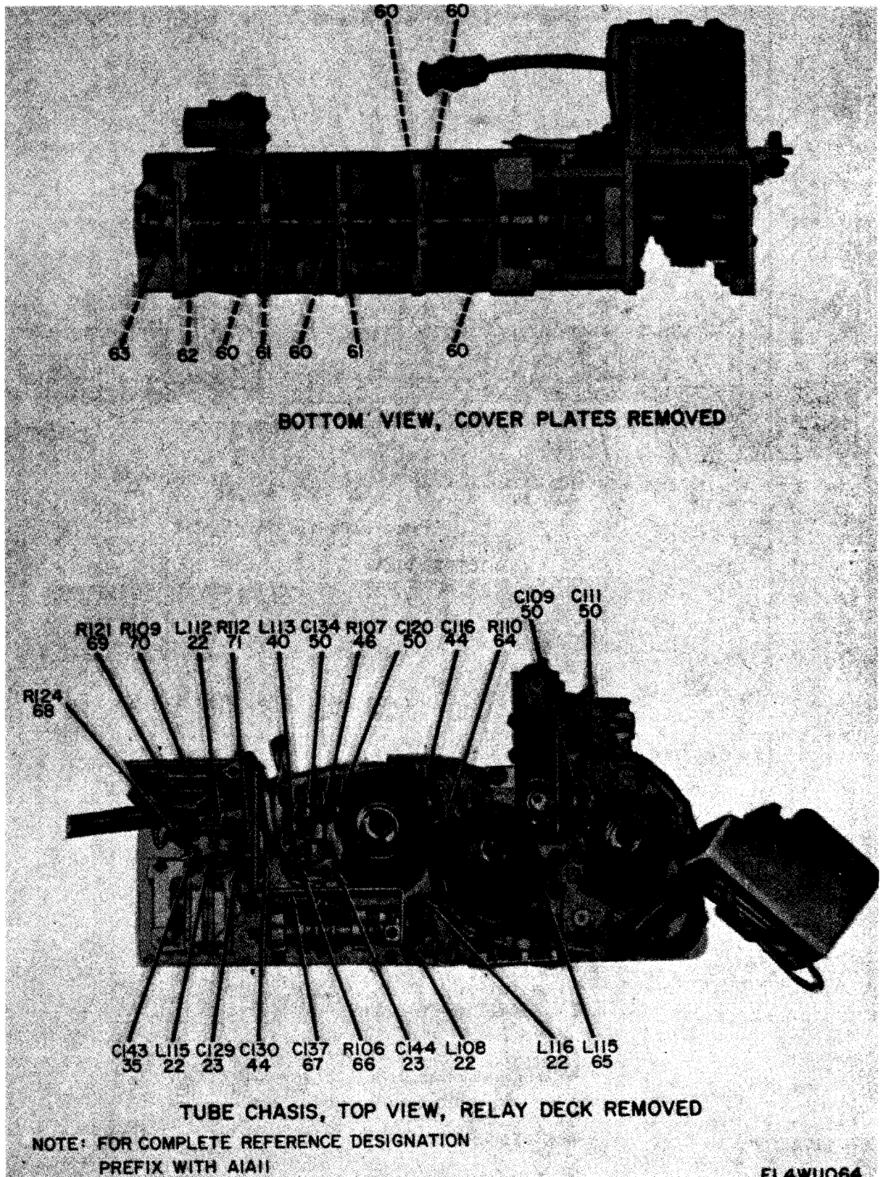
Figure 37. RF and Power Amplifier 225 to 399.9 MHz Subunit (A1A11) (Sheet 3 of 3).
