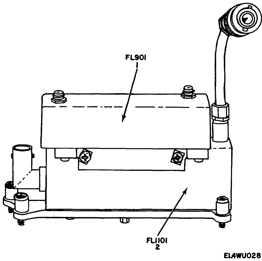
Figure 17. 500-kHz IF Filter and Low Pass Filter.
