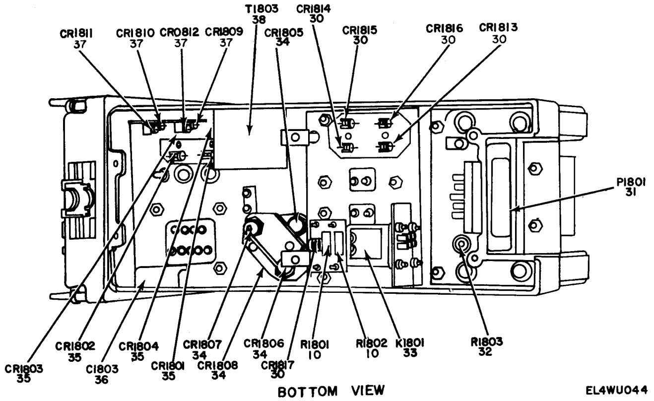
Figure 27. Power Supply PP-1494/U (Sheet 2 of 2).
