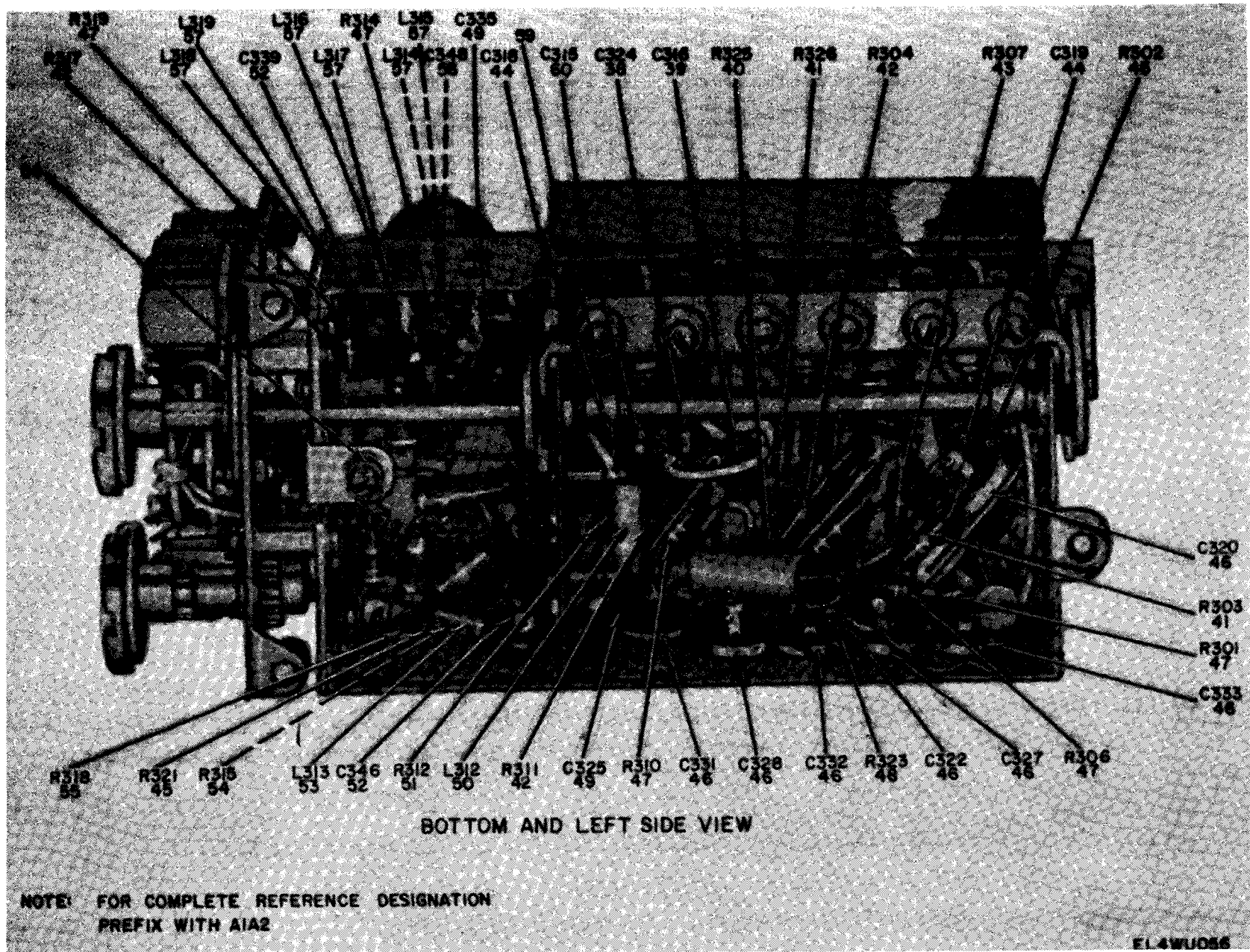
Figure 34. First IF Amplifier 20 to 29.9 MHz Subunit (A1A2) (Sheet 2 of 3).
