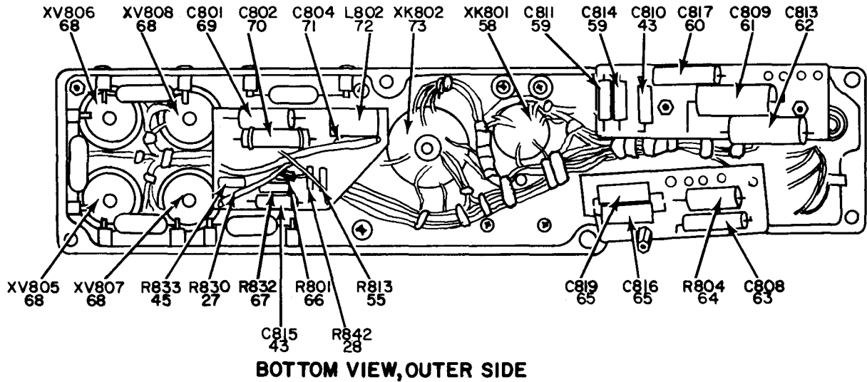
Figure 12. Audio Amplifier and Modulator, Subunit (A1A12) (Sheet 2 of 2).
