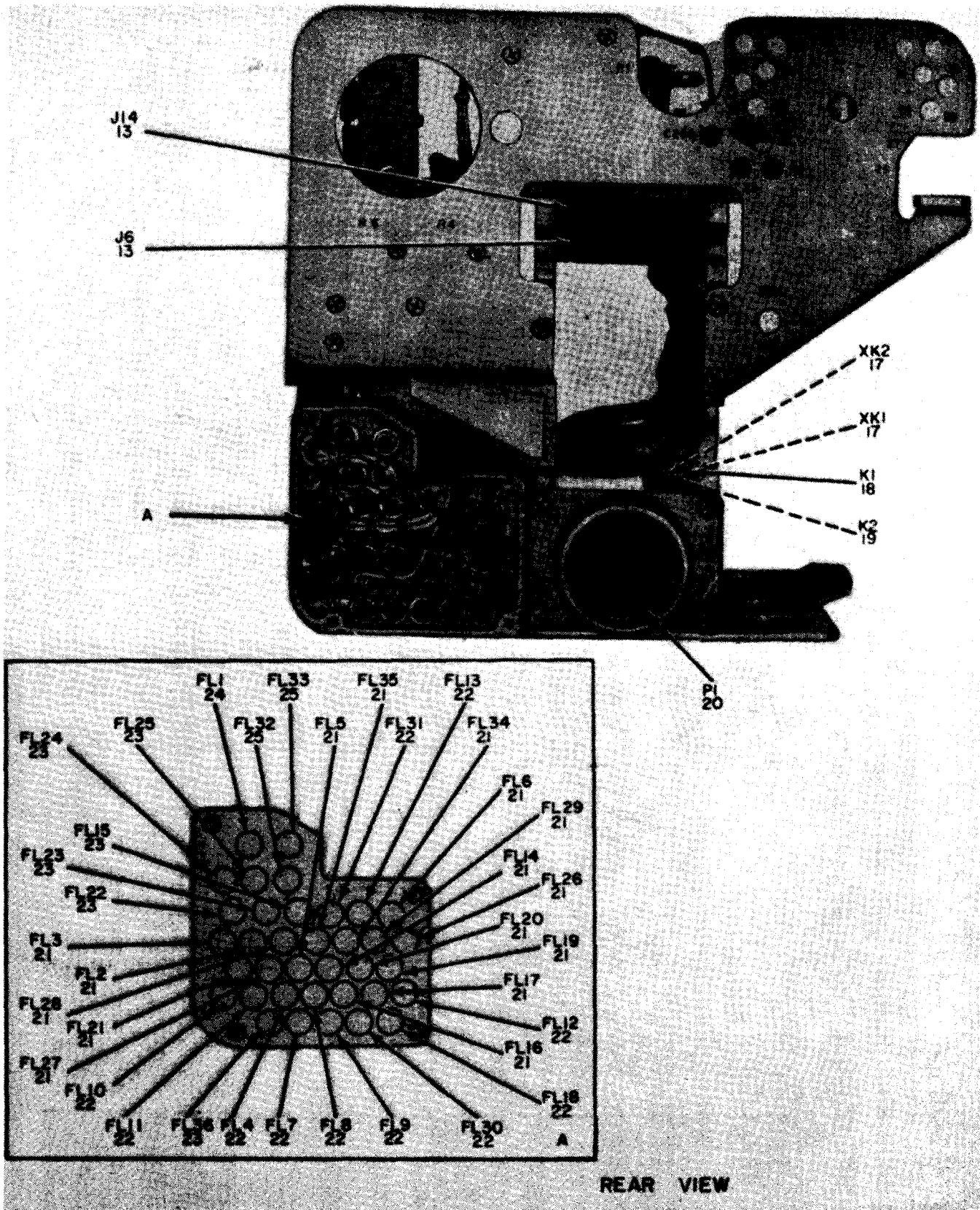
Figure 8. Receiver-Transmitters RT-323/VRC-24 and RT-323A/VRC-24 Main Frame (Sheet 2 of 2).
