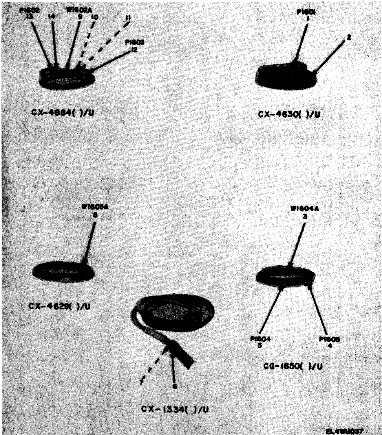
Figure 22. Cable Assemblies Group CG-1650( )/U, CX-1334( )/U, CX-4629( )/U, CX-4630( )/U, and CX-4884( )/U.
