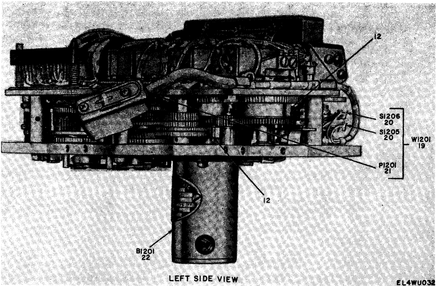
Figure 19. Frequency Selector Assembly (Sheet 3 of 4).
