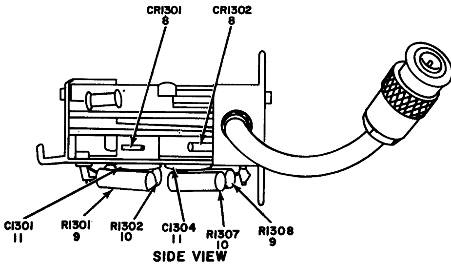
Figure 15. Coupler, Directional.
