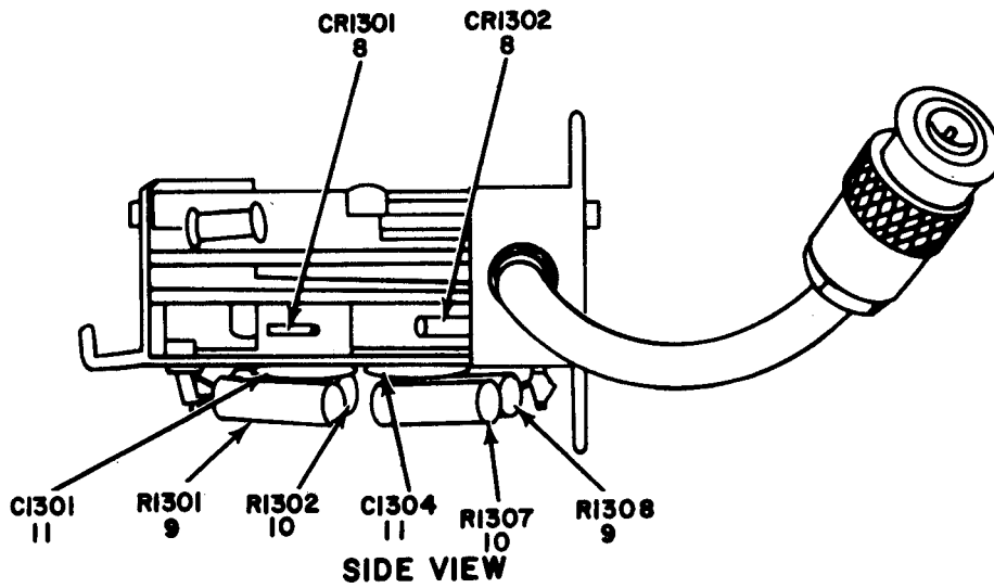
Figure 38. Coupler, Directional.
