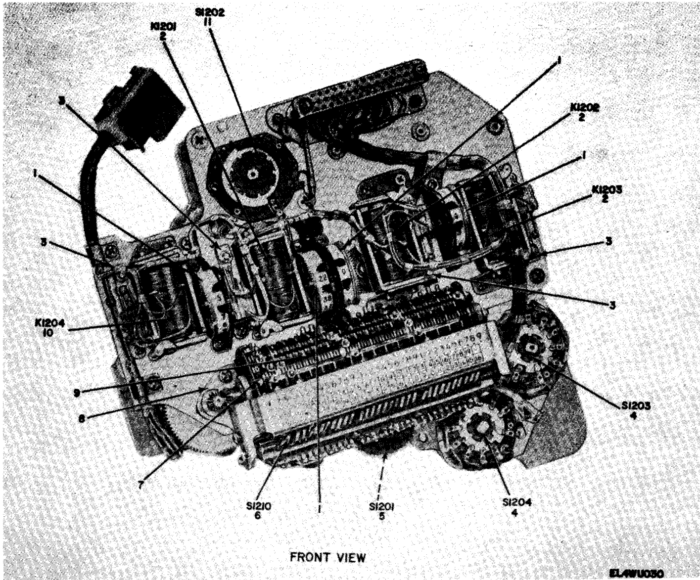
Figure 19. Frequency Selector Assembly (Sheet 1 of 4).
