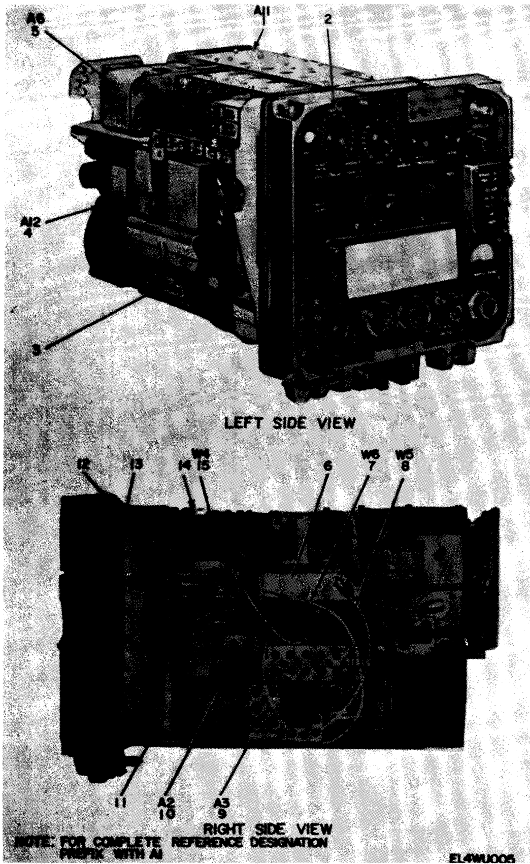
Figure 5. Receiver-Transmitters RT-323/VRC-24 and RT-323A/VRC-24 (Sheet 1 of 2).
