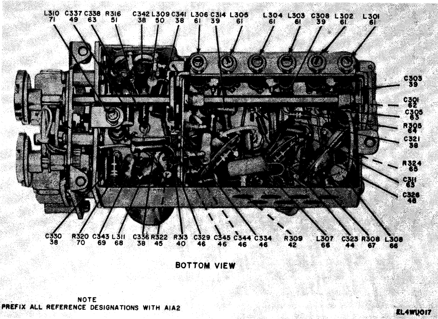
Figure 11. First IF Amplifier 20 to 29.9 MHz Subunit (A1A2) (Sheet 3 of 3).
