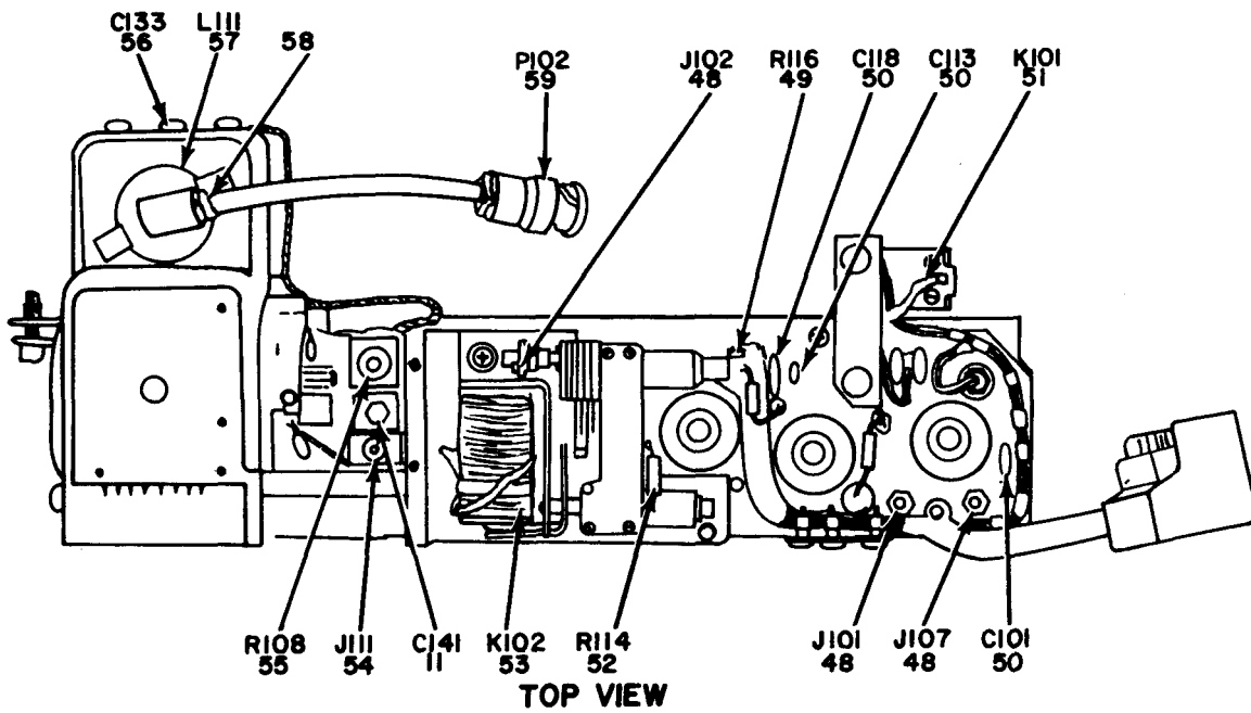
Figure 37. RF and Power Amplifier 225 to 399.9 MHz Subunit (A1A11) (Sheet 2 of 3).
